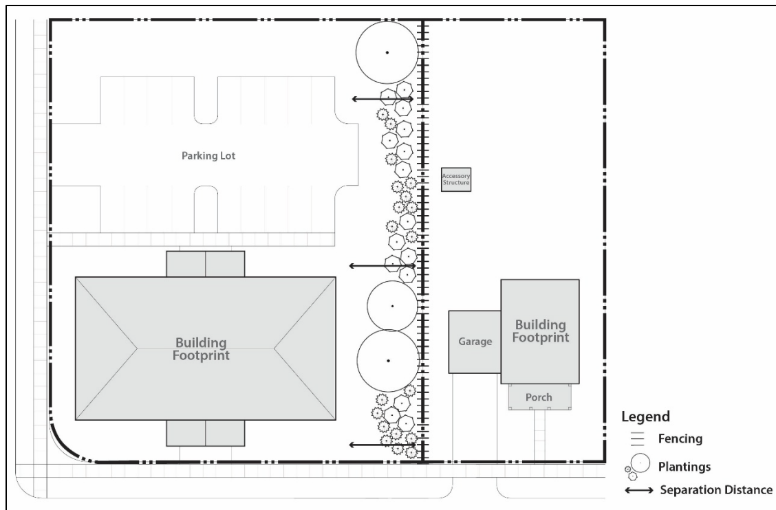
Figure 17.08.30h: Bufferyard Example
