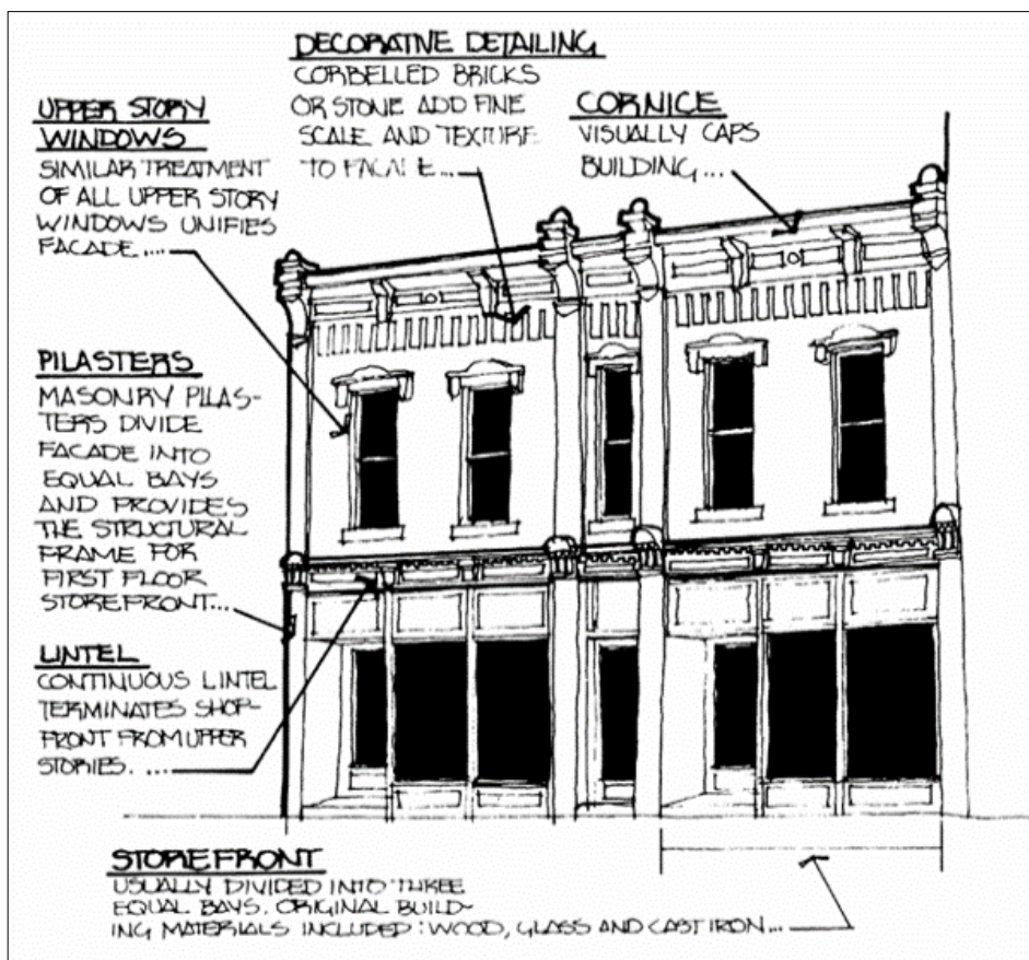
Figure 17.07.50a: Architectural Components
