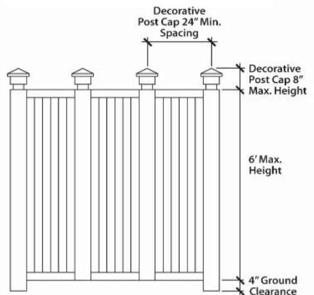
Figure 17.06.40b: Fence Measurements
