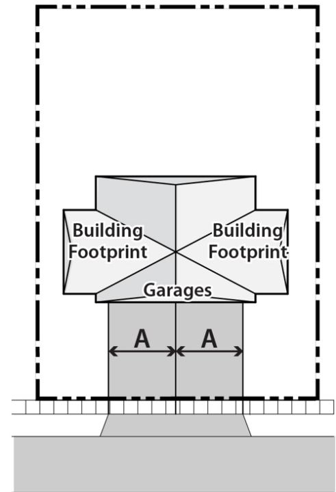
Figure 17.06.03d: Two Family Dwellings with Two Driveways
